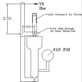
FIG 2 Minimum Geometry
